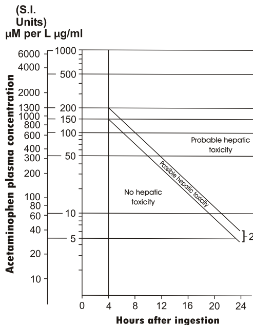
Figure 1. Rumack-Matthew Nomogram:
