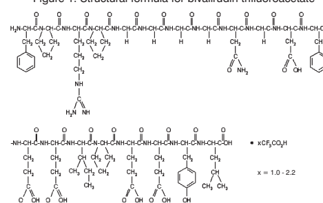
Figure 1. Structural formula for bivalirudin trifluoroacetate
